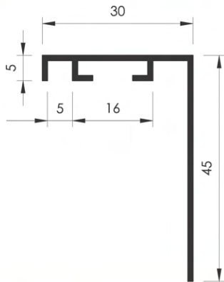
Frame Profile Section Exhaust and Fresh Air Louvers
