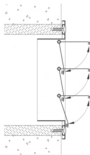
B. Face Screw Fixing The Gravity Louver is fixed to the wall (with wooden Frame) by means of visible screws.
