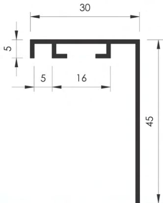
Frame Profile Section Gravity Louvers
