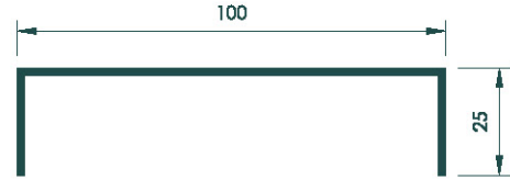
Blade Profile Section Sand Trap Louvers
