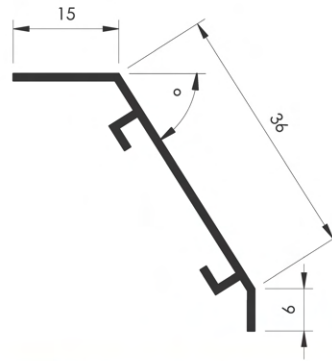
Louver Blade Profile Section Exhaust and Fresh Air Louvers
