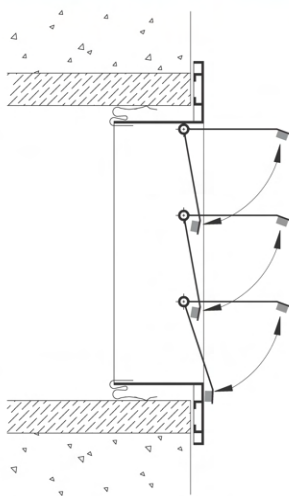
A. Concealed Fixing (Spring Clip Mounting) The Gravity Louver is fixed by means of spring clips to the wall or partition where no screws are visible.
